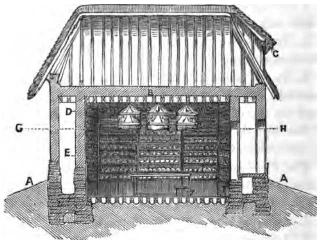
Fig. 188.—Elevation of Fruiterie, following the line K L, Fig. 189.
