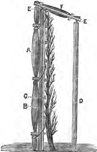
Fig. 173.—Cover for Apricots in Contra Espalier.
